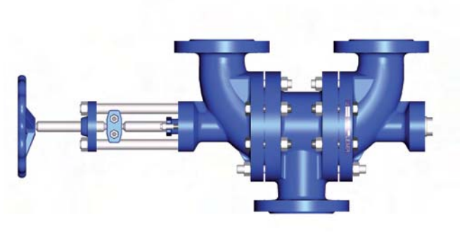
Type 310 Gland design
