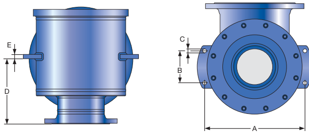
Support brackets
