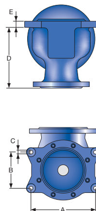
Support brackets
