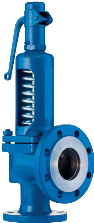
Type 442 Full nozzle Plain lever H3 Bonnet open Conventional design
